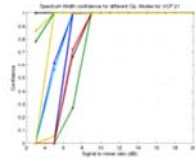
Different confidence maps based on SNR for various possible operational settings of NEXRAD VCP 21.
