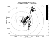
Clutter detected using REC on RCCG, 4/6/2012 10:31:47 Z, 0.5°
